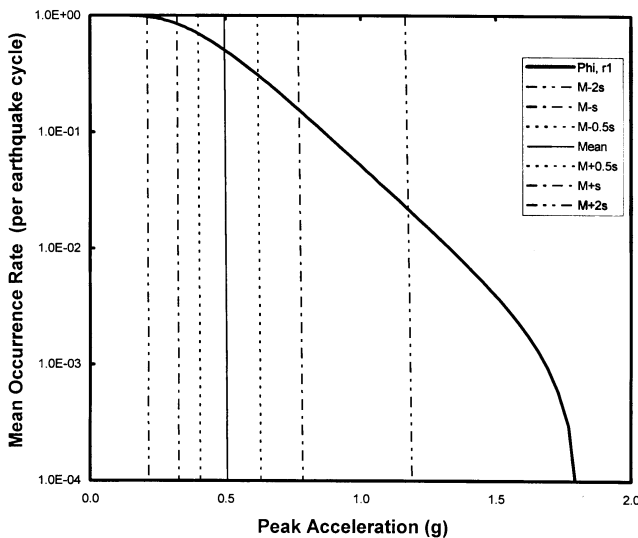
Figure 1. PSHA for a simplified case in which all of the hazard comes from a single fault which fails repeatedly in characteristic ground motion earthquakes, to illustrate the effects of the ergodic assumption. As in any PSHA, this gives hazard curves giving the mean occurrence rate of a ground motion (peak acceleration in this case). For clarity, the mean occurrence rate is given in repetitions per earthquake cycle, rather than per year as is normally done. The heavy line, ( \phi ) gives the result for a PSHA in which all of the uncertainty on the ground motion is treated as aleatory. The near-vertical lines represent the results of a PSHA in which all of the uncertainty is treated as epistemic. It is not known which of the vertical hazard curves to choose, but that weighting does not depend on the exposure time and thus the overall estimate of hazard also does not depend on exposure time.
