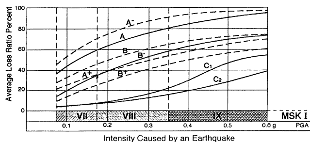
Figure 2. Vulnerability functions for various building types vs the earthquake intensities. A: Buildings in field stone, rural buildings, unburnt brick houses, clay house (1 to 1 ½storey); B: Ordinary brick buildings, buildings in large blocks, half timbered buildings in natural dressed stone (1 to 1 ½storeys); C 1 : Buildings in strengthened masonry in cement (1 to 2 storeys); C 2 : Reinforced concrete and steel buildings, well built wooden buildings; A - : A type, but taller (2 or more storeys); A + : A type, earthquake-resistance features; B - : B type, but taller (2 or more storeys); B + : B type with earthquake-resistance features.
