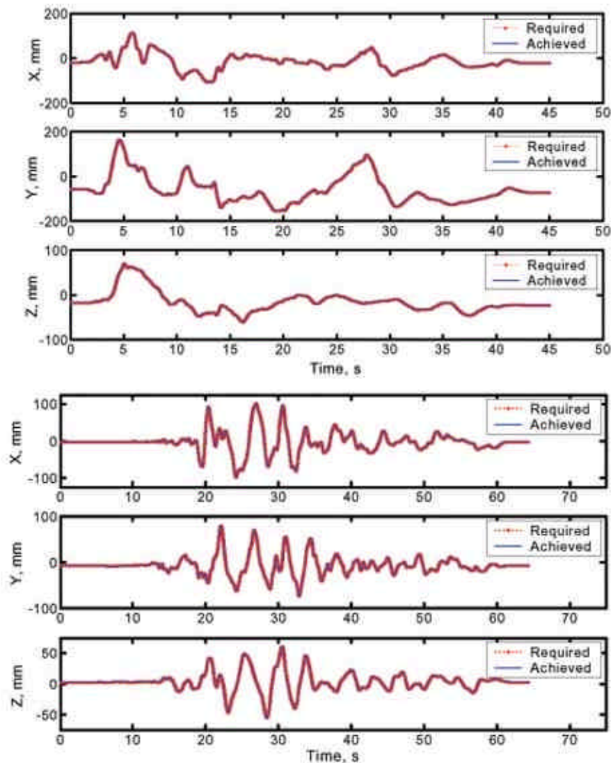
Figure 7. Three-axis table response computed from actuator position. (Top) El Centro (bottom) Chi-Chi. These are ‘first shot’ responses with payload after initial tuning without payload under harmonic movement.
