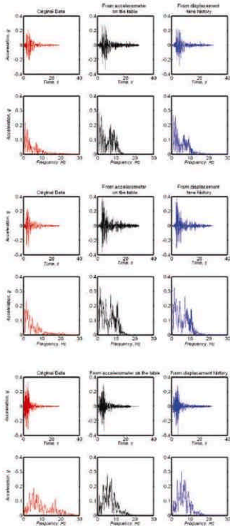
Figure 10. X (top), Y (middle) and Z (bottom) table response to Kalamata spectrum.
