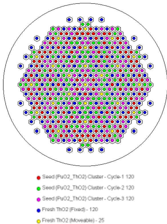
Figure 9. ATBR equilibrium core 120 FAs/batch – 720 EFPD. Schematic diagram of the three-batch fuels and thoria clusters.
