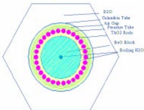
Figure 2. Typical arrangement of seedless thoria cluster.
