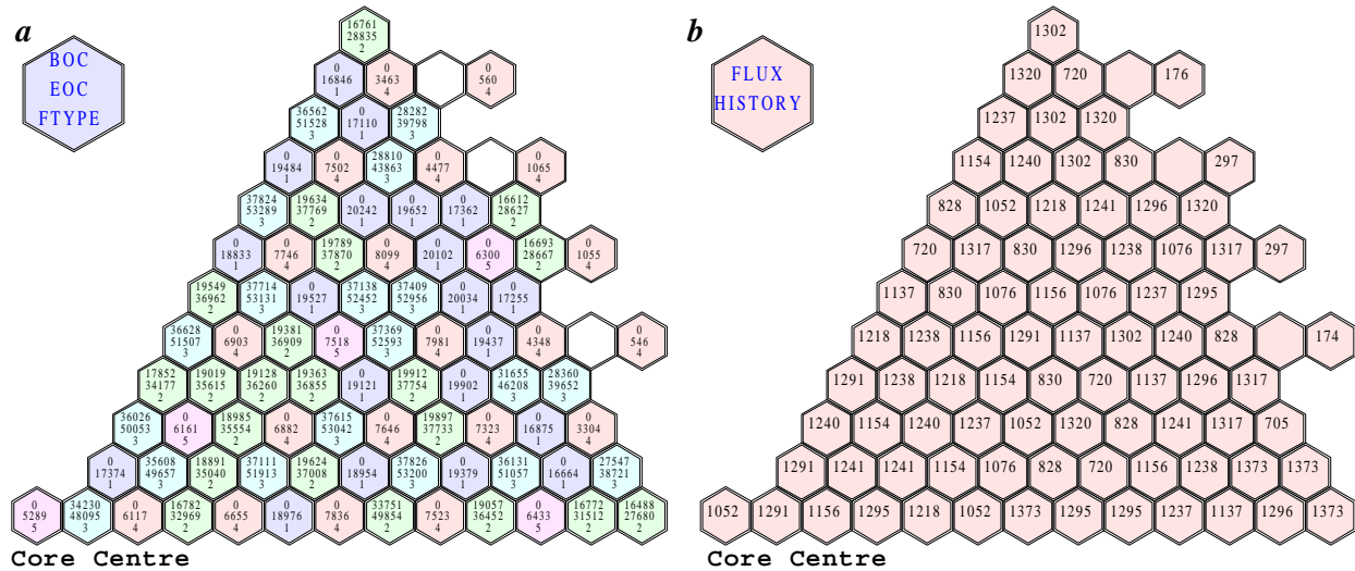
Figure 8 a, b. a , ATBR one-sixth equilibrium core 120 FAs per batch – BOC/EOC burn-up distribution (MWD/T). FTYPE: 1. (fresh) Cycle-1; 2. Cycle-2; 3. (last) Cycle-3; 4. Fixed thoria cluster; 5. Moveable thoria cluster. b , One-group absolute flux history values in units of 10^{11} n/cm 2 /s (Core average value = 1.118 \times 10^{14} n/cm 2 /s) k_{\infty} of thoria cluster after irradiation at different flux levels.
