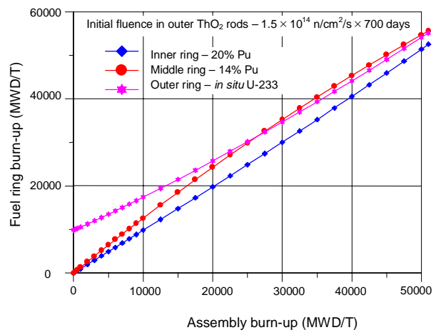
Figure 7. Burn-up accumulation in the three rings of seed fuel cluster.
