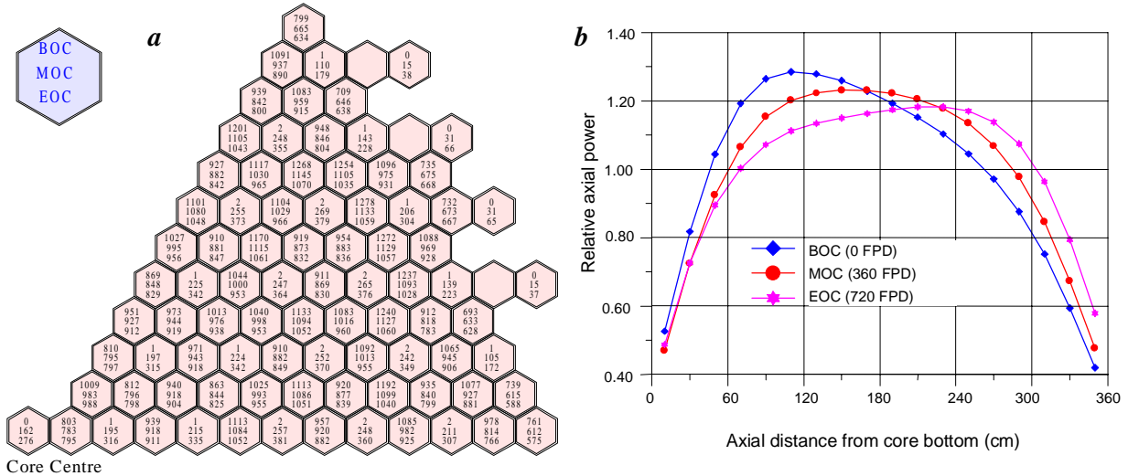
Figure 11 a, b. a, ATBR one-sixth equilibrium core 120 FAs/batch-radial power distributions at BOC/MOC/EOC. The radial power distribution given here is relative power in each fuel assembly. They are multiplied by 1000 to print in integer format. A value of 1000 means it is average relative power = 1.0. BOC/MOC/EOC, Beginning/middle/end of fuel cycle. b, ATBR-600 equilibrium core with PuO_2 seed in ThO_2 . Axial power distribution at BOC/MOC/EOC.
